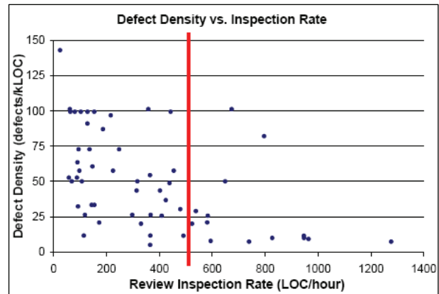
Figure 1: Inspection effectiveness falls off when greater than 500 lines of code are under review.
